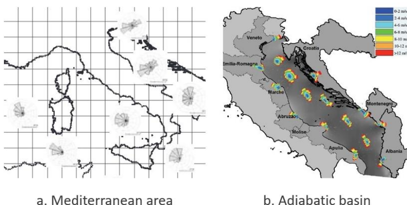
Figure 28. Wind frequency distribution (Sources: Lavagnini et. al., 2006, POWERED project)
