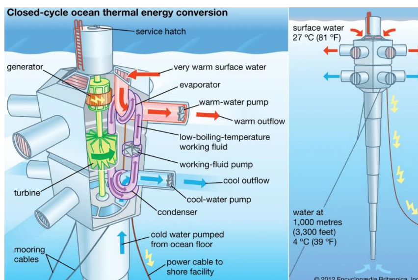
Figure 9. Illustration of OTEC cycle 15
