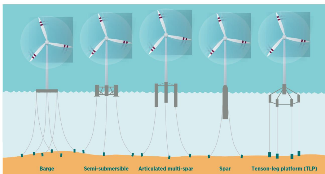
Figure 6. Main categories of floating offshore wind turbine foundations (Source: IRENA 2021a)
