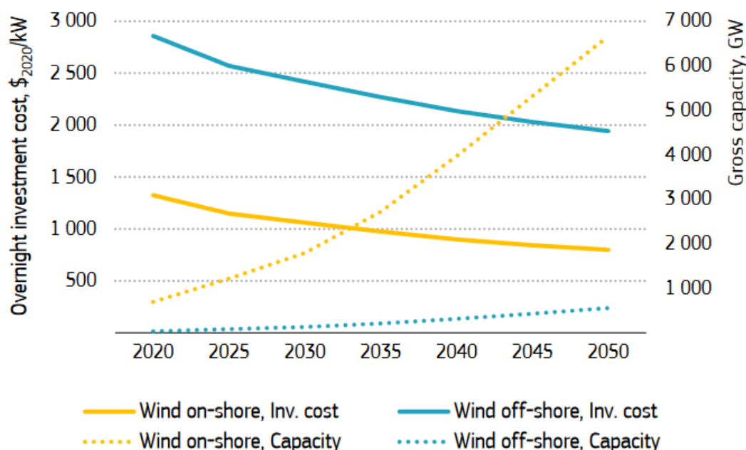
Figure 15. Overnight investment costs (in USD) for onshore and offshore installations according to the POLES-JRC model (Source: JRC, 2023)
