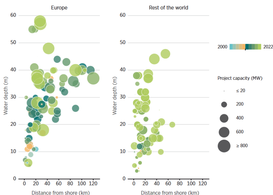
Figure 12. Offshore wind turbine development trends, 2000-2022 (Source: IRENA, 2023b)
